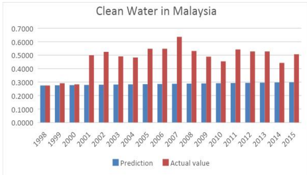
Fig. 3. Graph of prediction and actual value for clean water in Malaysia using discrete dynamical system
