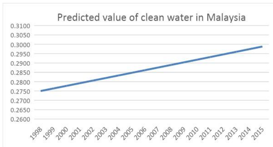
Fig. 1. Graph of predicted value of clean water in Malaysia
