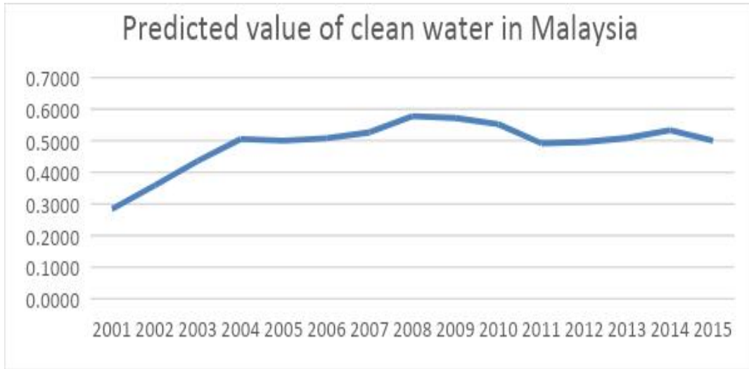
Fig. 2. Forecasted value of clean water in Malaysia by using moving average method
