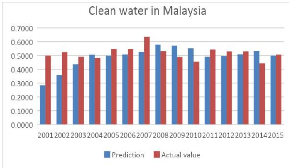
Fig. 4. Graph of prediction and actual value for clean water in Malaysia using time series analysis
