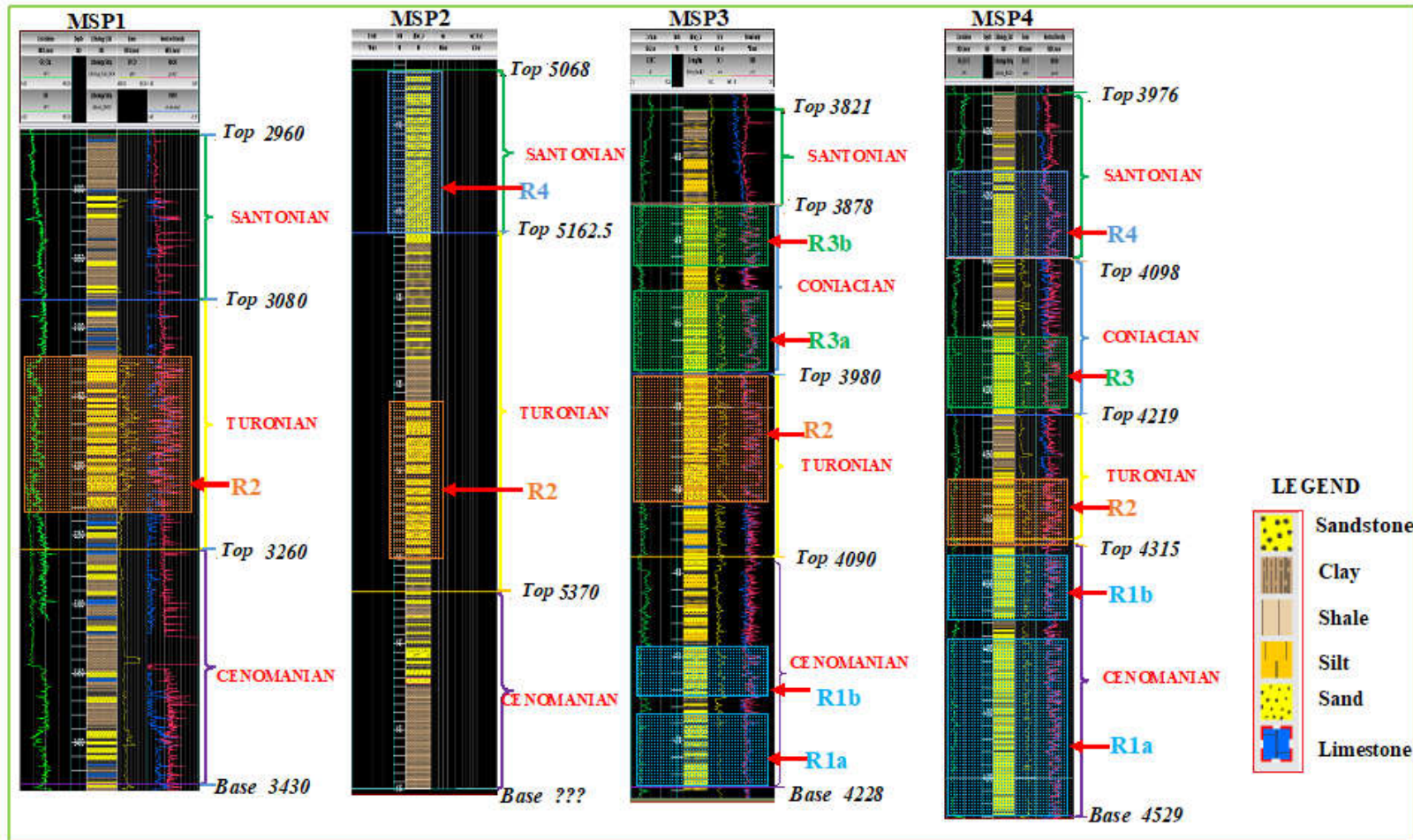
Fig. 6. Lithostratigraphic log of the different wells studied
