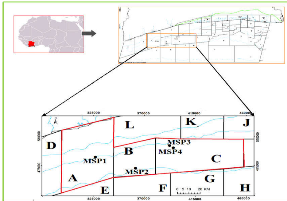
Fig. 2. Location of the wells
