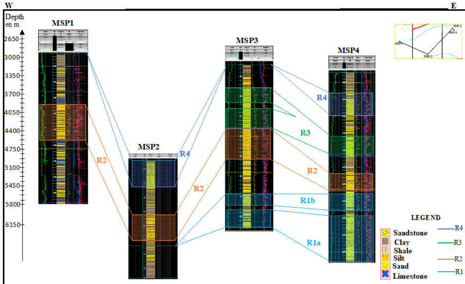
Fig. 7. West-East Correlation profile of wells reservoirs studied
