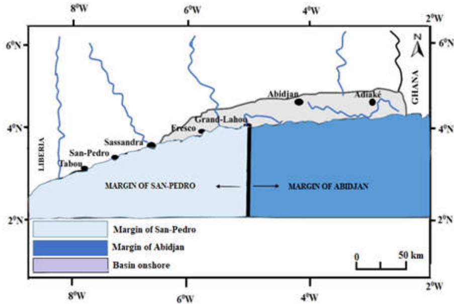
Fig. 1. Margins of the sedimentary basin of Côte d'Ivoire
