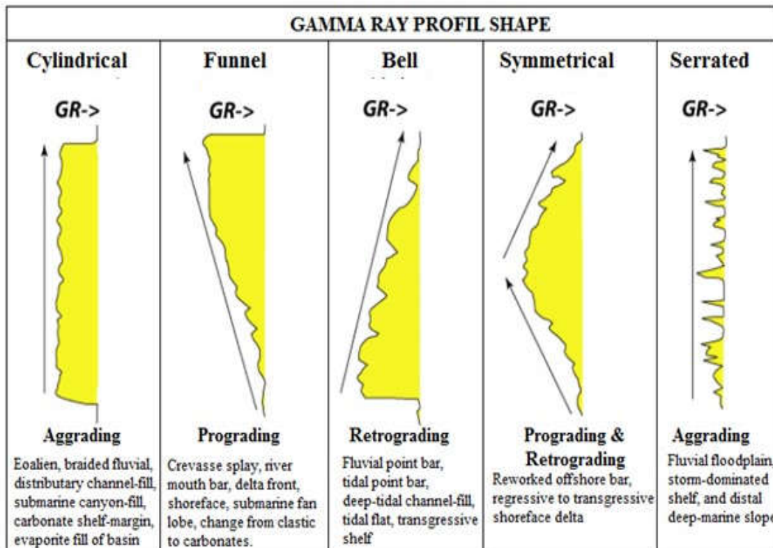
Fig. 3. Standard gamma ray (GR) response model based on variation in grain size and deposit environments [9]
