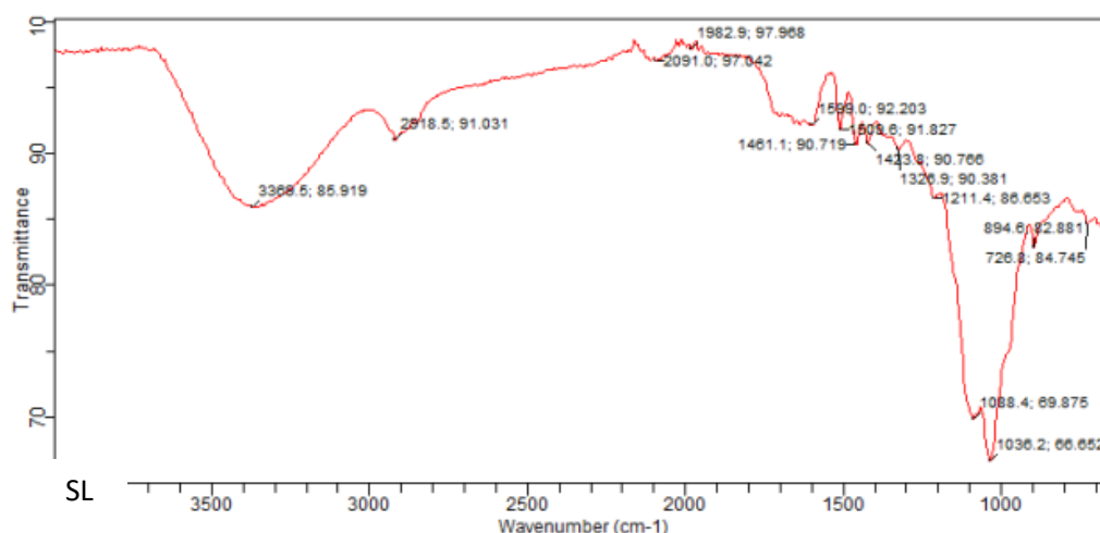
Fig. 2. FTIR spectrum of soda lignin
