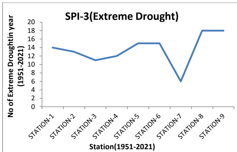
Fig. 3. 3-month SPI of extreme drought for Punpun-Harohar basin
