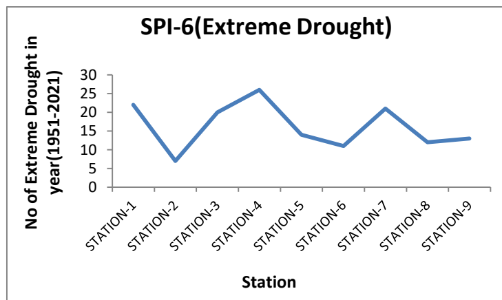
Fig. 4. 6- month SPI of extreme drought for Punpun-Harohar basin
