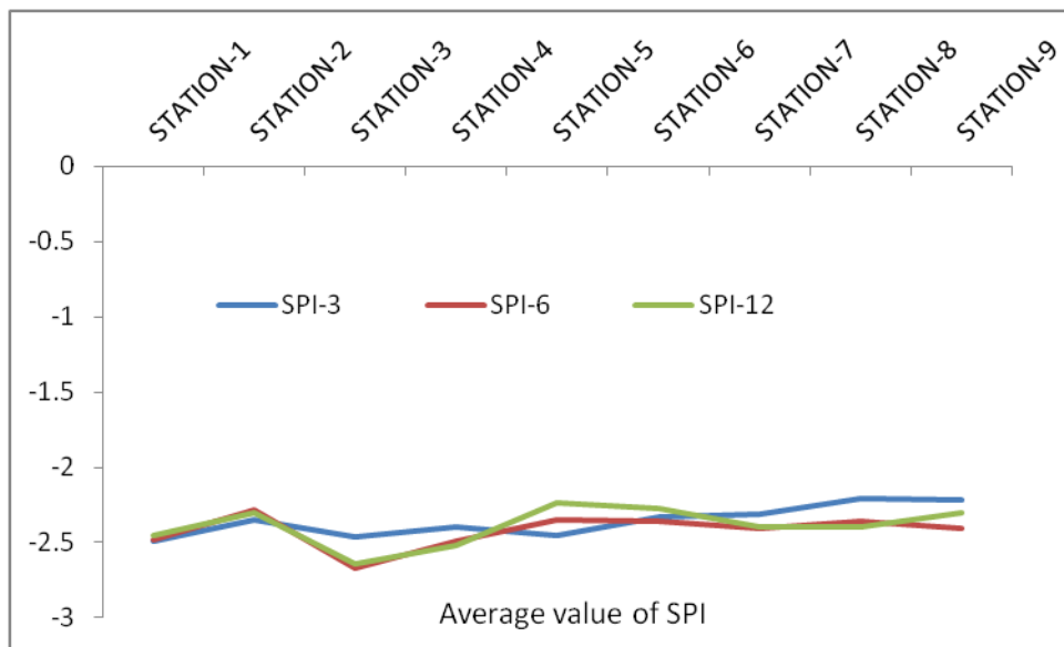
Fig. 8. 3, 6 & 12- month SPI of extreme drought for Punpun-Harohar basin
