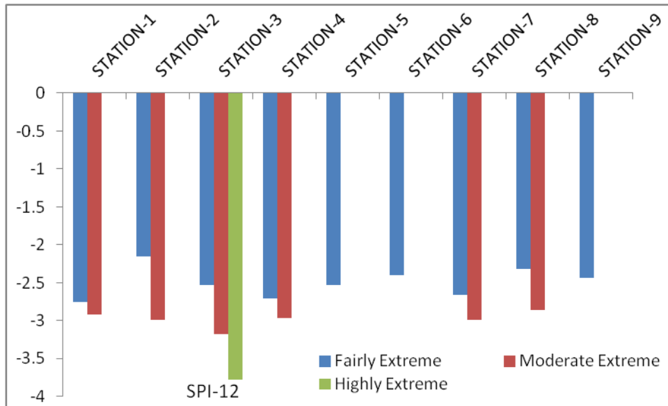
Fig. 7. 12- month SPI of different extreme drought for Punpun-Harohar basin
