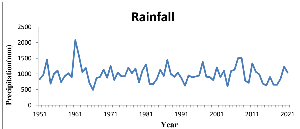
Fig. 2. Yearly precipitation (mm) from 1951 to 2021 for Punpun-Harohar basin
