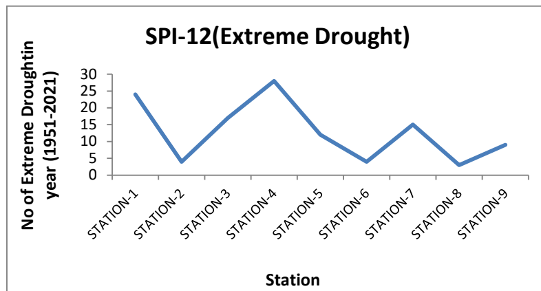
Fig. 5. 12- month SPI of extreme drought for Punpun-Harohar basin
