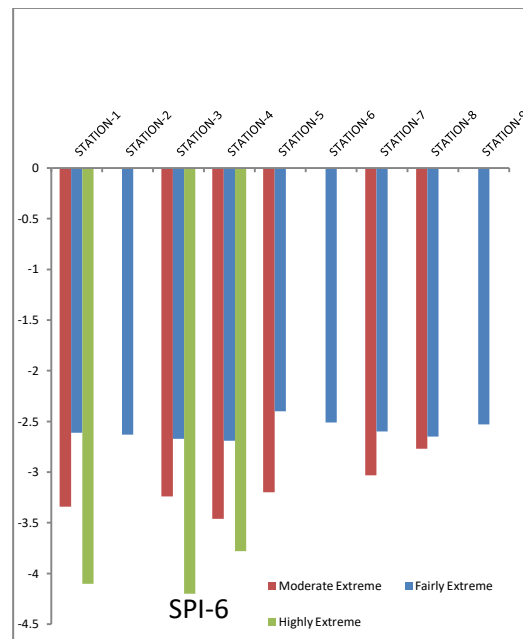
Fig. 6. 3 & 6- month SPI of different extreme drought for Punpun-Harohar basin
