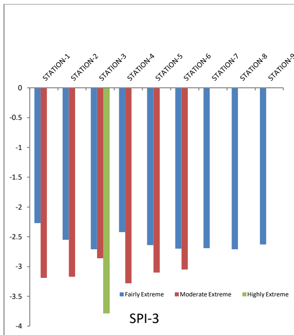
Fig. 6. 3 & 6- month SPI of different extreme drought for Punpun-Harohar basin
