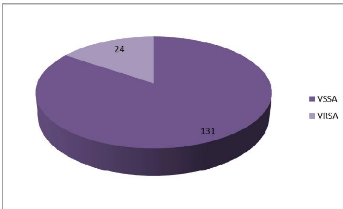
Fig. 1. Abundance of Staphylococcus aureus and VRSA recovered in the study
