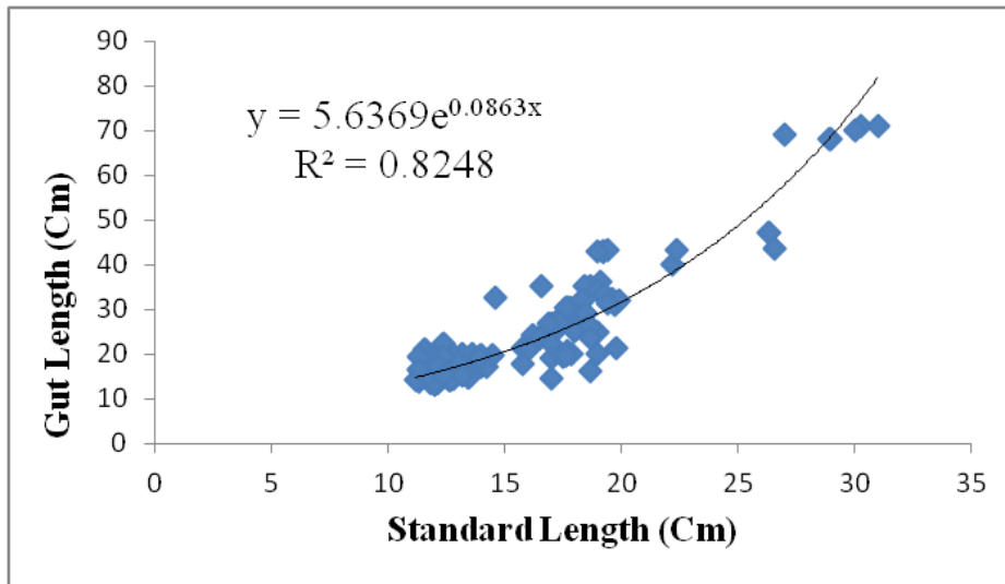
Fig. 2. Length- length relationship (LLR) of Schilbe mystus
