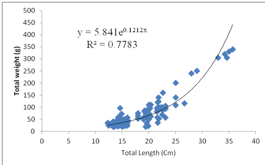
Fig. 1. Length-weight relationship (LWR) of Schilbe mystus
