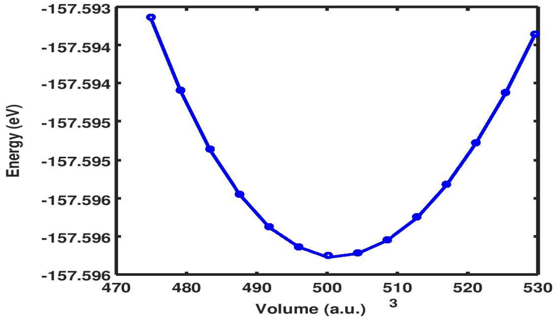
Fig. 2. Calculated total energy and volume of NiTe 2 using GGA
