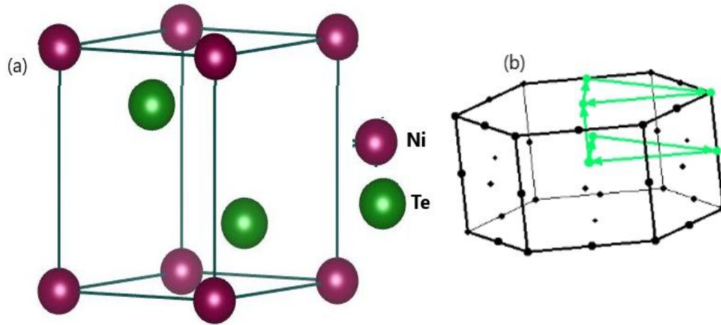
Fig. 1. (a) Vesta view of NiTe 2 and (b) First brillouin zone of NiTe 2 from xcrystden
