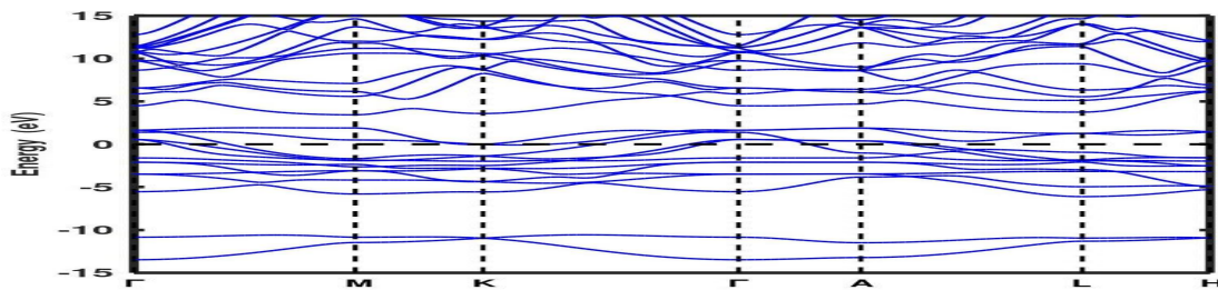
Fig. 3. Computed electronic band structure of NiTe 2 using GGA
