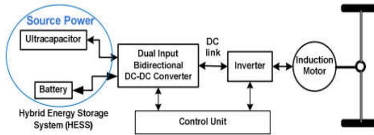
Fig. 3. Block diagram of power circuit of EV with HESS
