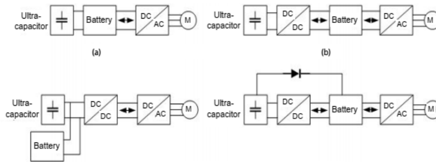
Fig. 6. A direct parallel connection of ultracapacitor with battery; b Bi-directional DC-to-DC converter balancing the power flow between ultracapacitor and battery
