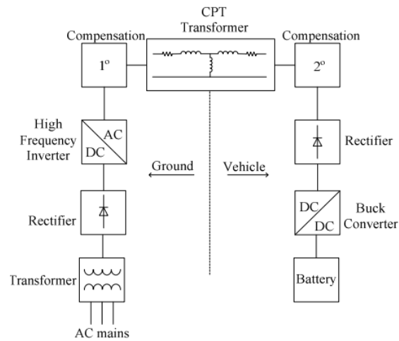
Fig. 5. Structure of a CPT system
