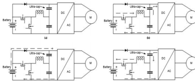
Fig. 7. Hybrid energy storage using ultracapacitors (a) Basic topology (b) Battery power flow to the motor during acceleration (c) Constant speed power flow (d) Retardation power flow
