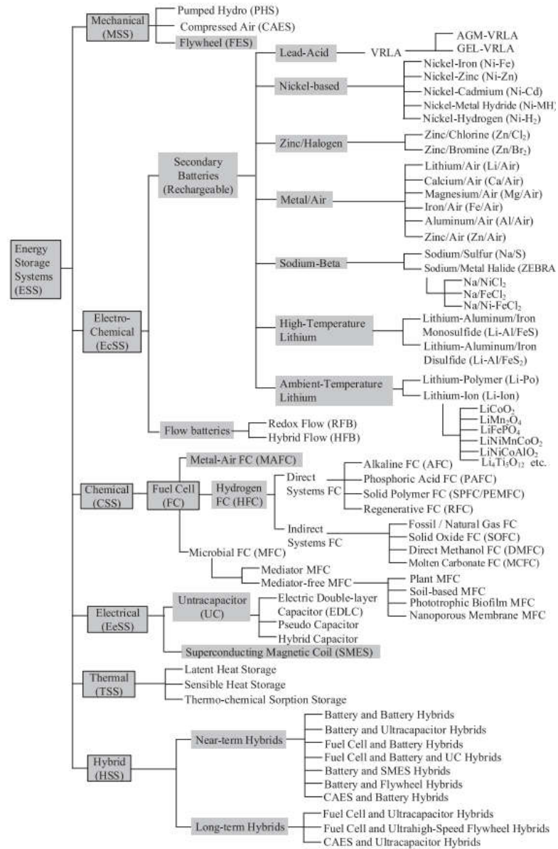
Fig. 4. ESS based on composition material and energy formation [1]
