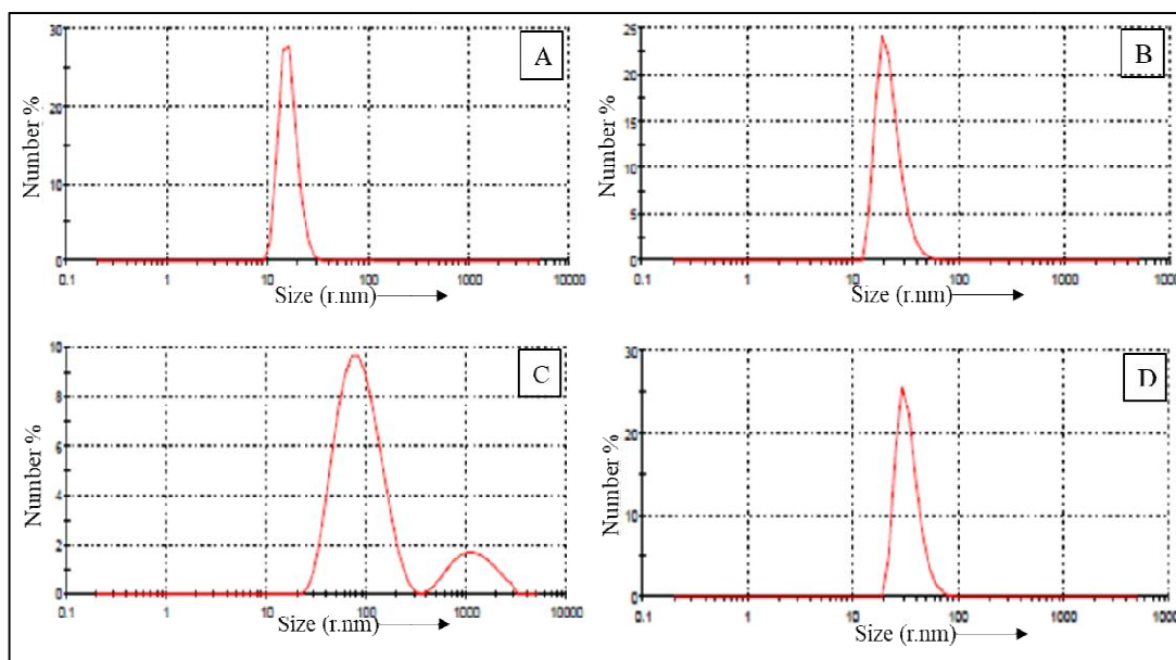
Fig. 2. Particle size analyser (PSA) image of synthesized silver nanoparticles of (A) Abroma augusta (B) Barringtonia acutangula (C) Dillenia indica (D) Eupatorium odoratum
