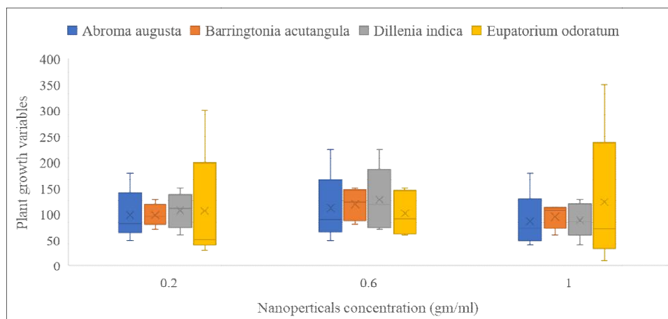
Fig. 4. Box & whisker plot of different plant growth variables with synthesized silver nanoparticles
