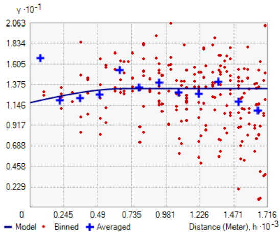
Available S
