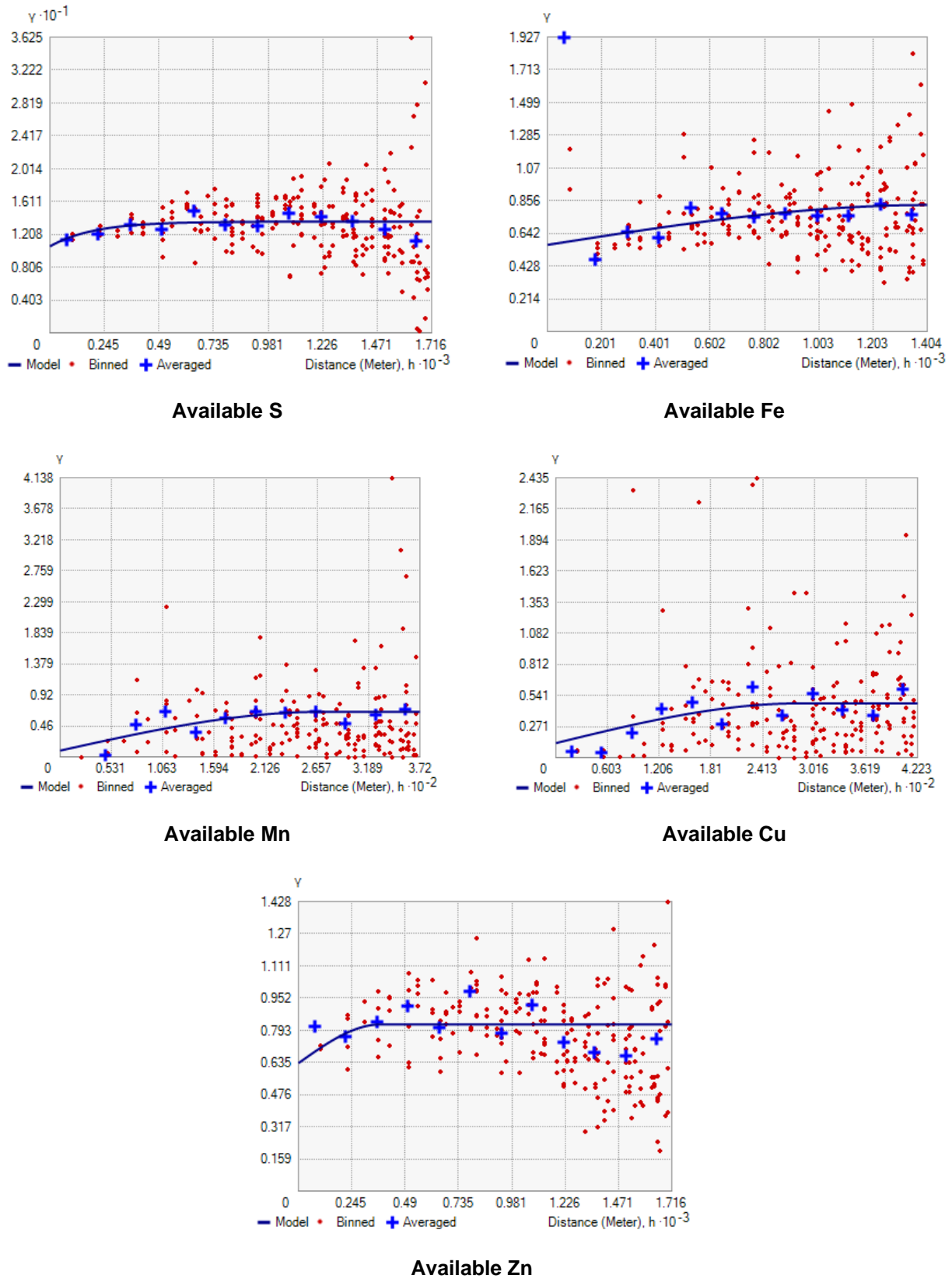
Fig. 3. Semi variograms and fitted models of sub surface soil properties
