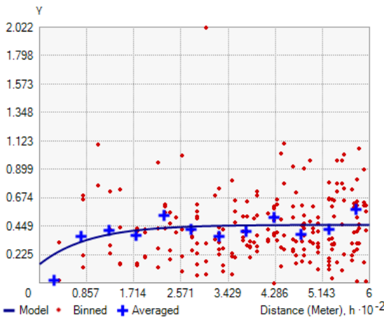
Available Mn
