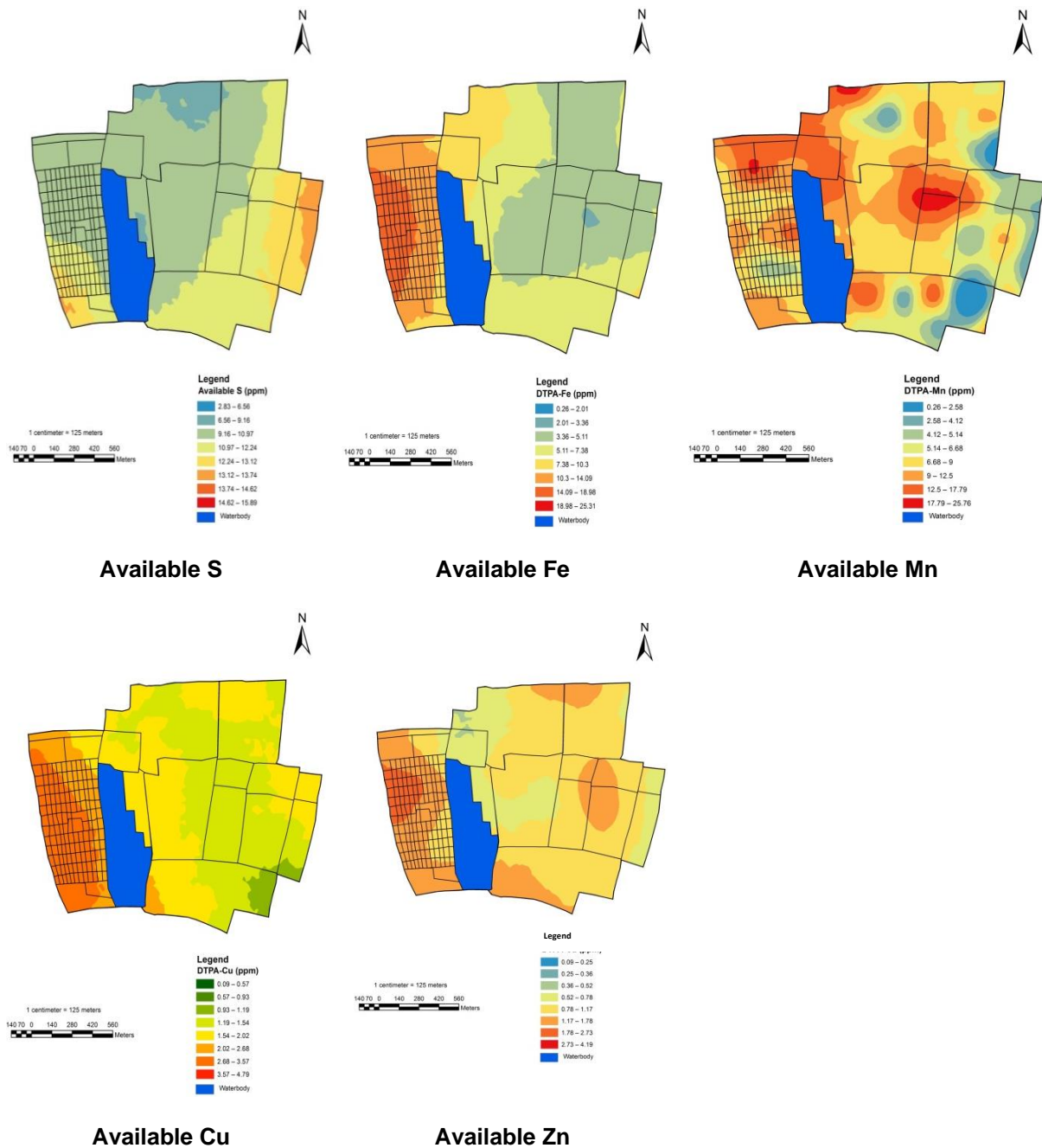
Fig. 5. Soil map of spatial distribution of nutrients for sub surface soil in the study area
