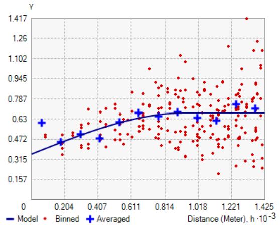
Available Fe
