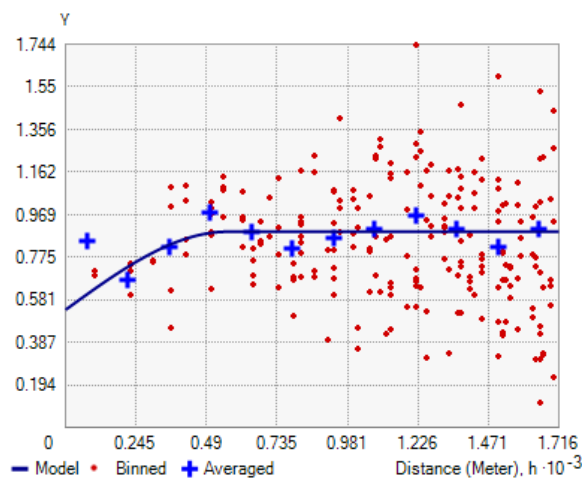
Available Zn
