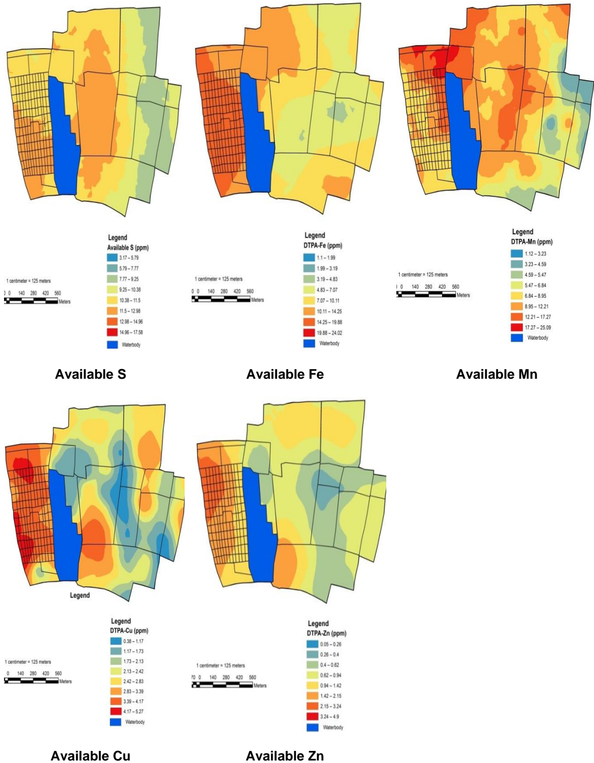
Fig. 4. Soil map of spatial distribution of nutrients for surface soil in the study area
