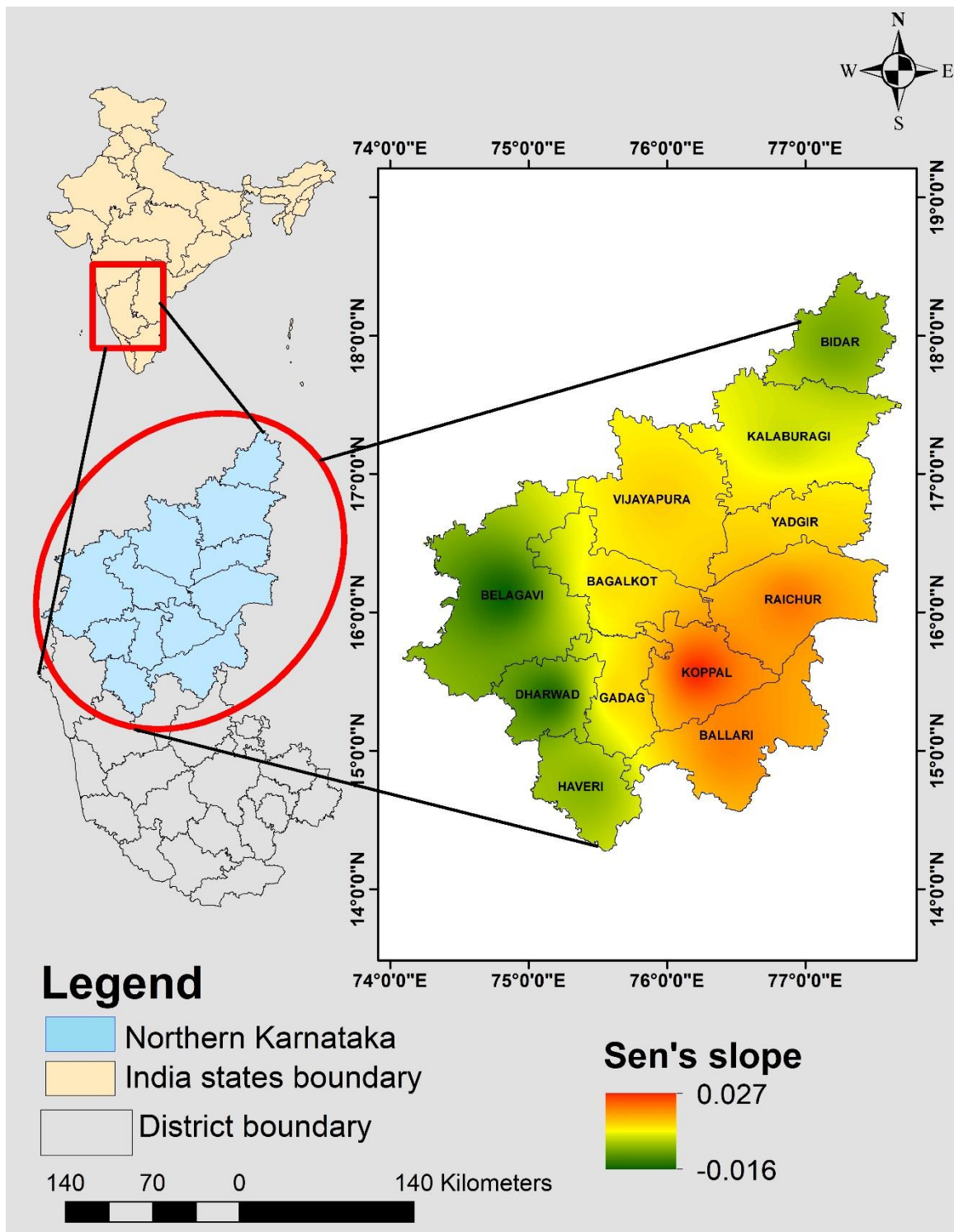
Fig. 1. Spatial map of Sen's slope trend magnitude
