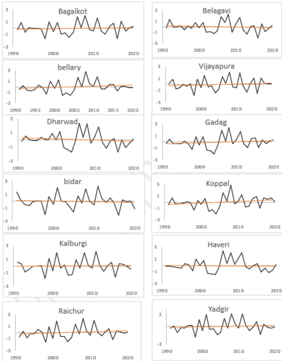
Fig. 2. SPI-3 trend of Northern Karnataka districts
