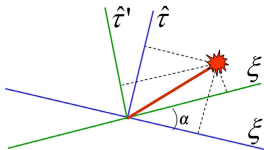
Figure 2. Mutual rotation of Cartesian coordinate systems [7] \xi, \hat{t} and \xi', \hat{t}' .
