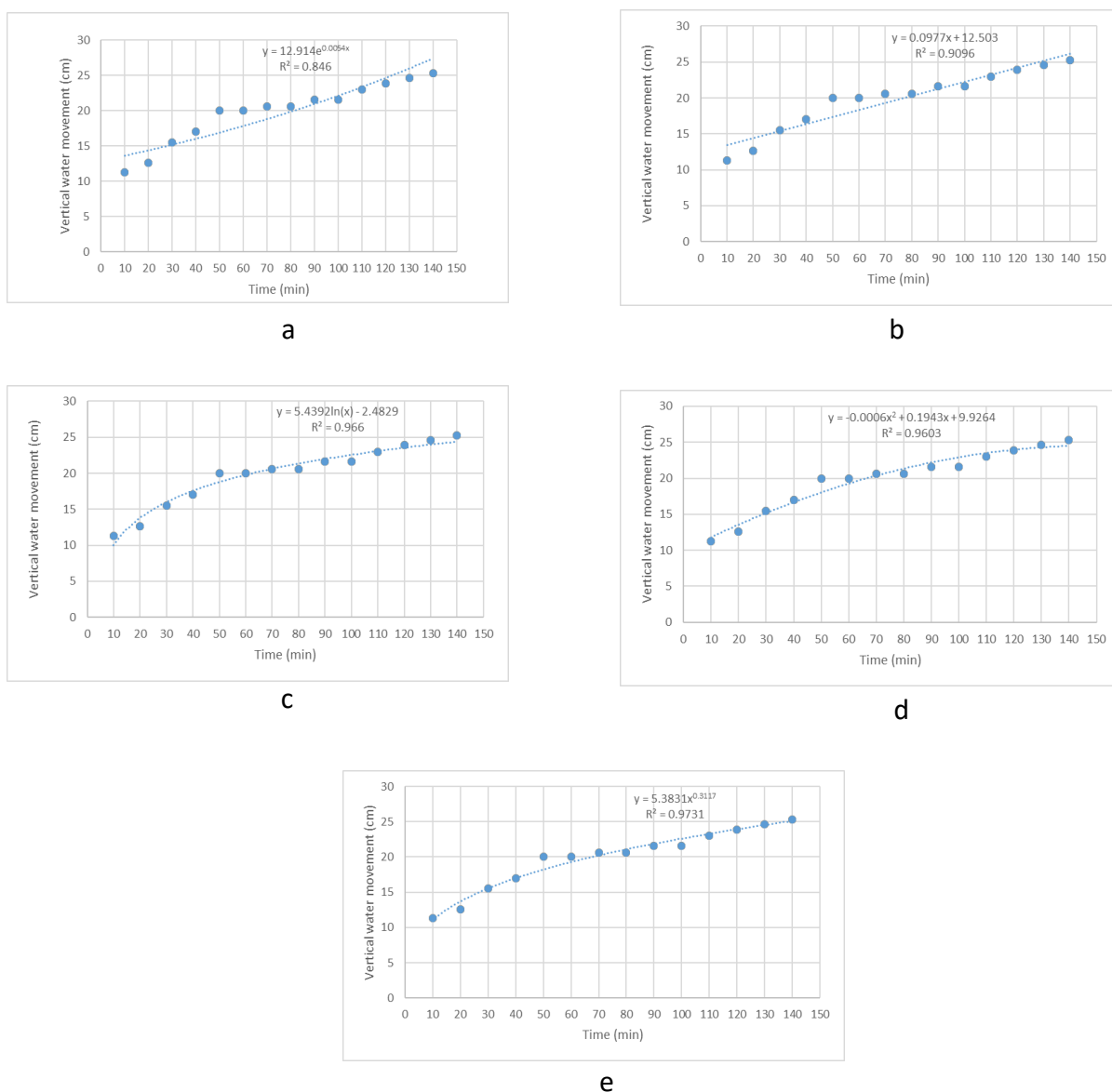
Graph 1. Based on Observed Vertical Measurement data during wetting pattern in the field Statistical Modeling for (a) Exponential Model, (b) Linear Model, (c) Logarithmic Model, (d) Polynomial model, (e) Power Model
