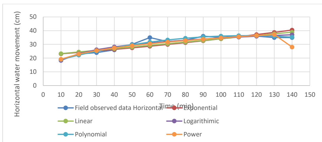
Graph 4. Comparison of observed wetting pattern in Horizontal path with statistical models
