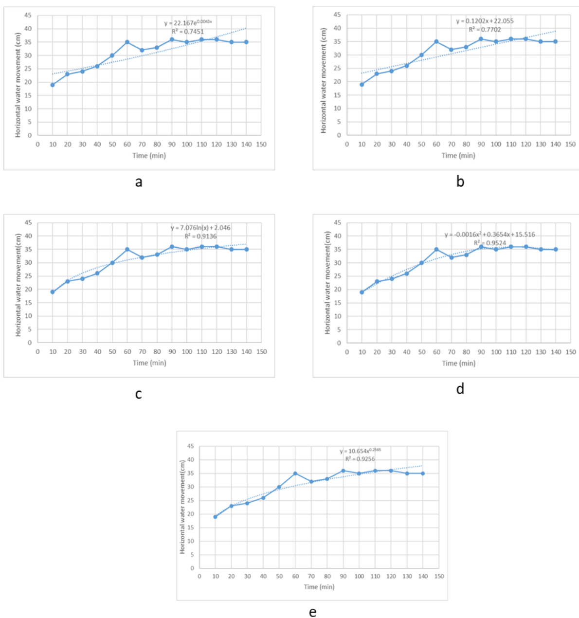
Graph 2. Based on Observed Horizontal Measurement data during wetting pattern in the field Statistical Modeling for (a) Exponential Model, (b) Linear Model, (c) Logarithmic Model, (d) Polynomial model, (e) Power Model
