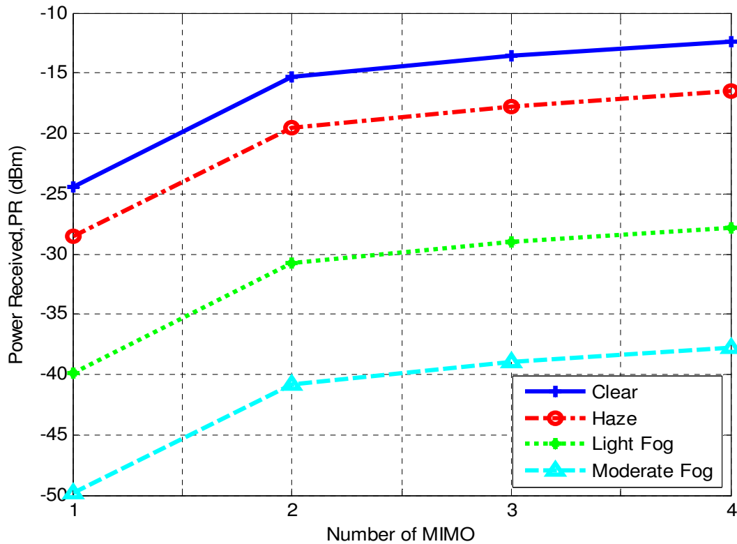
Fig. 3. Received power vs. size of MIMO system in different weather conditions
