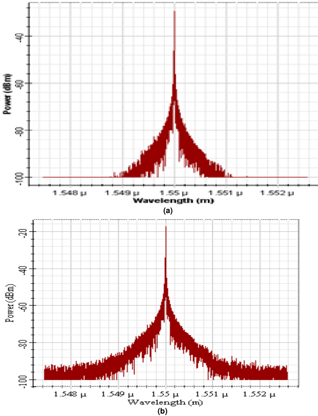
Fig. 6. Signal power at receiver for haze weather condition a)SISO b)4x4 MIMO
