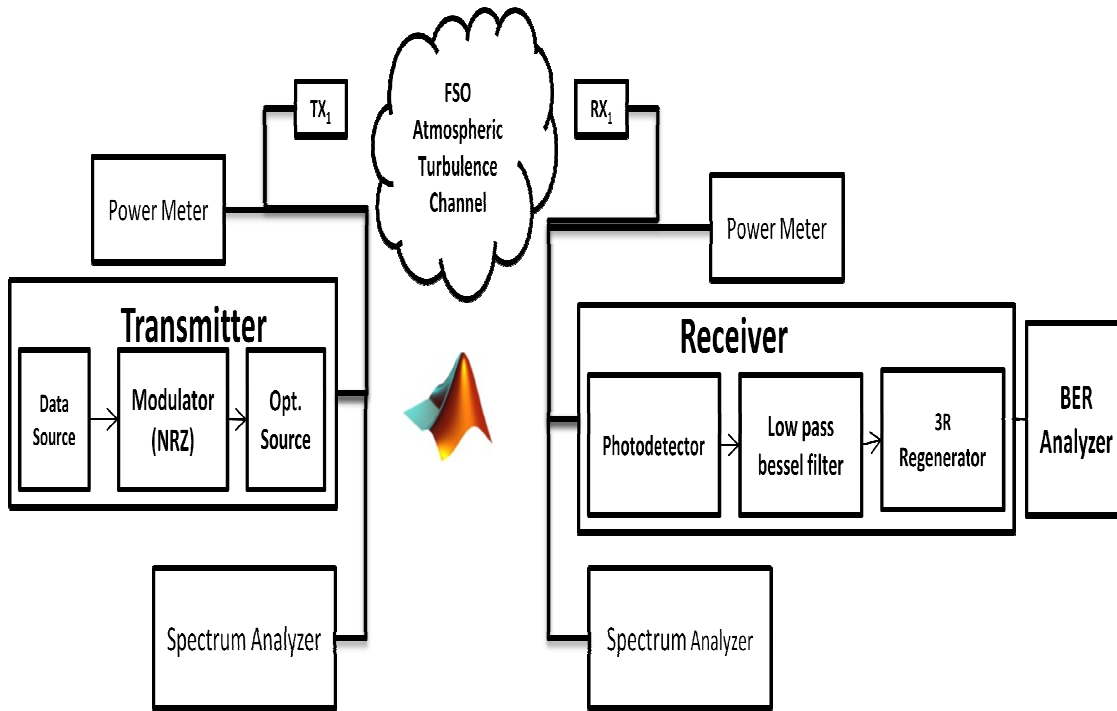
Fig. 2. Design model of Single-Input Single-Output free space optical system
