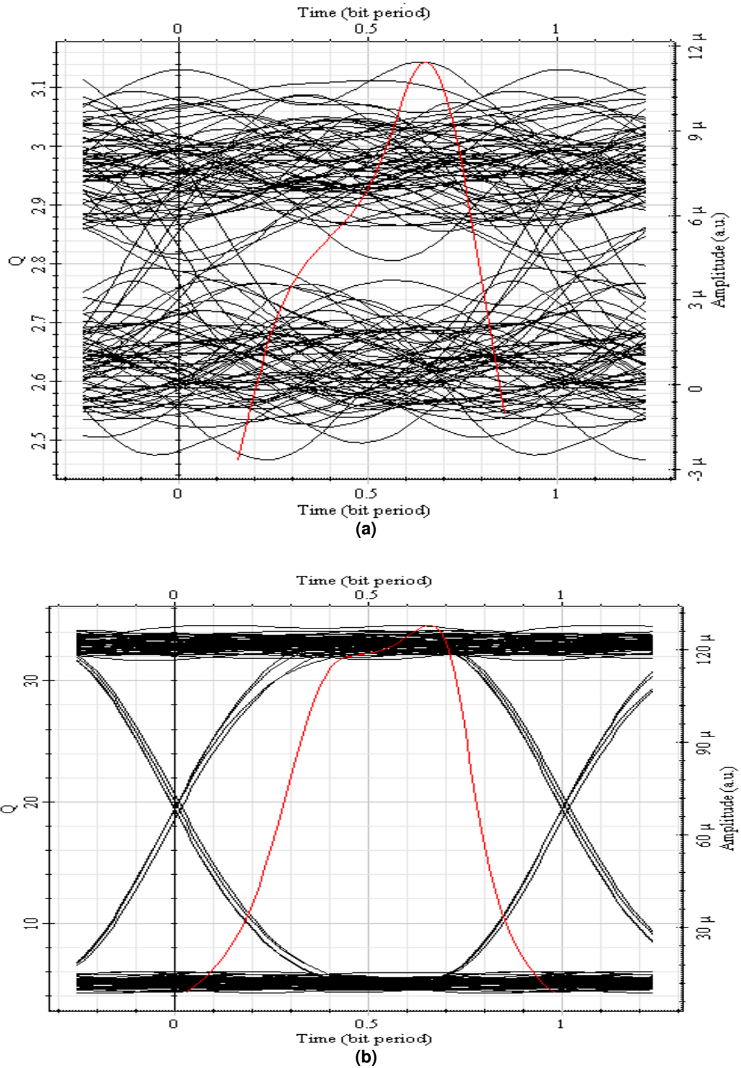
Fig. 5. Eye diagram for haze weather condition (a) SISO (b) 4x4 MIMO
